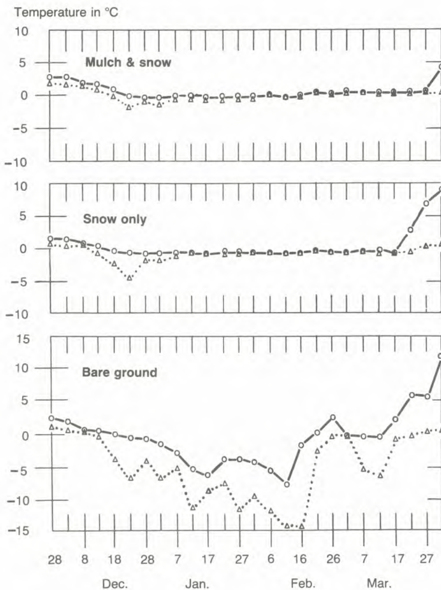
Figure 1 —Five-day minimum and maximum soil temperatures for nurserybed plots having mulch plus snow cover, snow cover only, or bare ground during the winter of 1981-82. Soil temperatures were taken at a depth of 13 centimeters.
