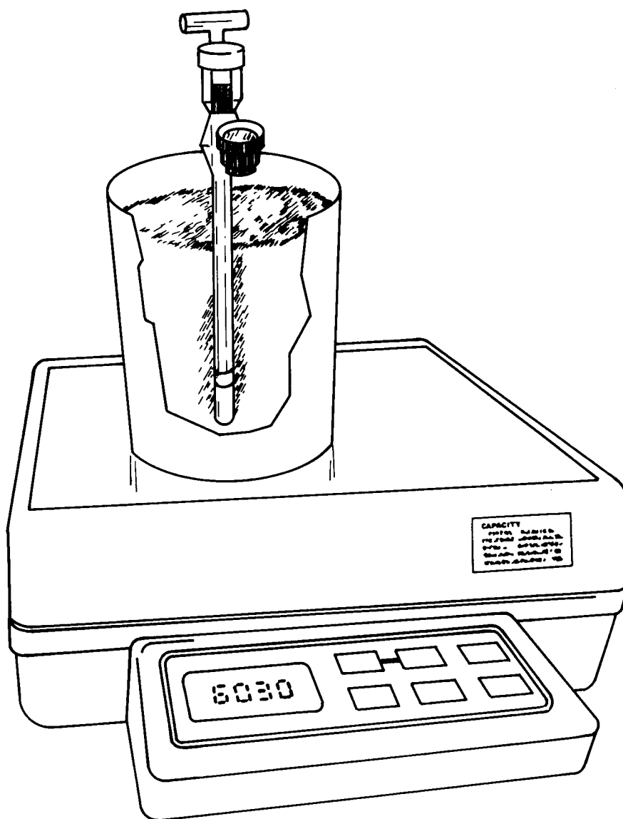
Figure 1—Weighing the pot and tensiometer.
