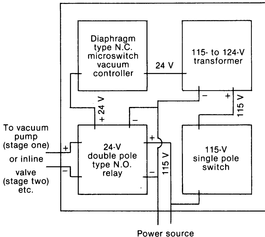
Figure 3—Electrical control panel for soil moisture stress chambers.
