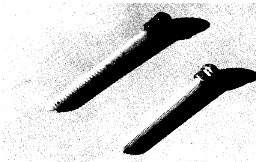
Figure 3—Lag screw with domed hex nut head.
