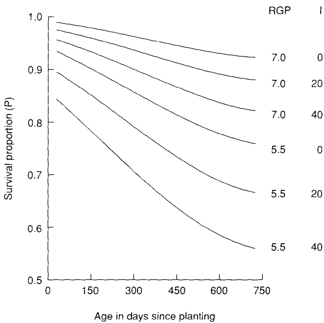
Figure 2 — Predicted survival proportion on the Shasta-Trinity National Forest. RGP = root growth potential and l = the product of the number of days in the first growing season when the average daily surface temperature exceeds 30 °C and the percentage mortality from the root exposure test.
