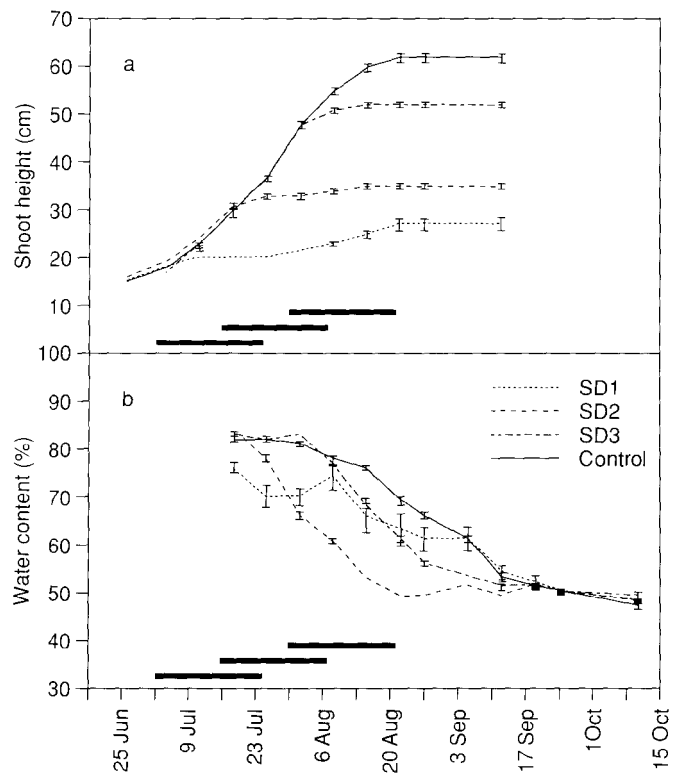
Figure 1 — Mean weekly height growth (a) and water content (b) of the uppermost 5 cm of silver birch seedlings in short-day (SD)-treated and control seedlings during the autumn 1995. The vertical bars are the standard errors of the means. Horizontal bars indicate blackout treatments.
