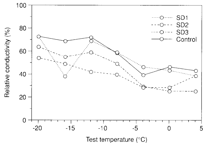
Figure 2 — Relative conductivity values after the first freezing test at 7 test temperatures on August 28–29, 1995. Lower values indicate greater cold hardiness. Each symbol is the mean of 2 independent samples (2 seedlings).
