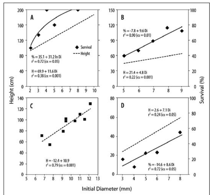
Figure 1. Relationship between initial seedling diameter and survival and height after 26 mo of (A) Cupressus lindleyii at San Bartolo Ameyalco, (B) Pinus ayacahuite v. veitchii at San Banabé Ocoatepec, (C) Pinus ayacahuite v. veitchii at Rancho Don Nati (height only), and (D) Pinus patula at Los Mena.
